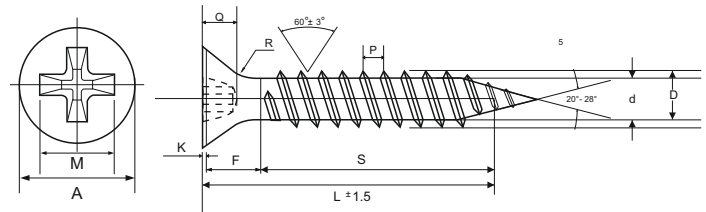
Dimension Drawing
