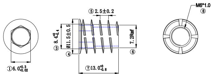
Hex Metal socket M6x13
